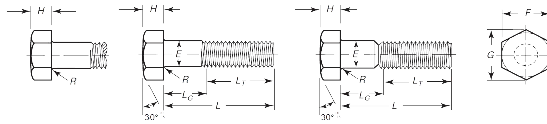
Bolt With Reduced Diameter Body
